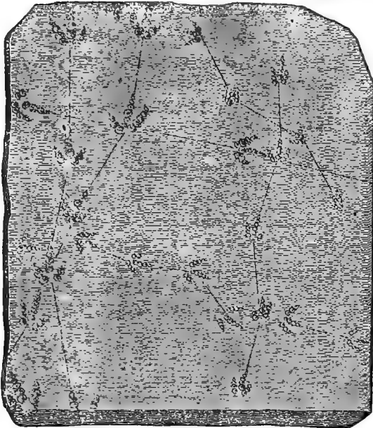
BIRD TRACKS OF THE CONNECTICUT.
